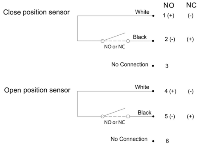
Figure 27: VSPZ – 2 wire "Z" proximity switch (NO/NC programmable)
